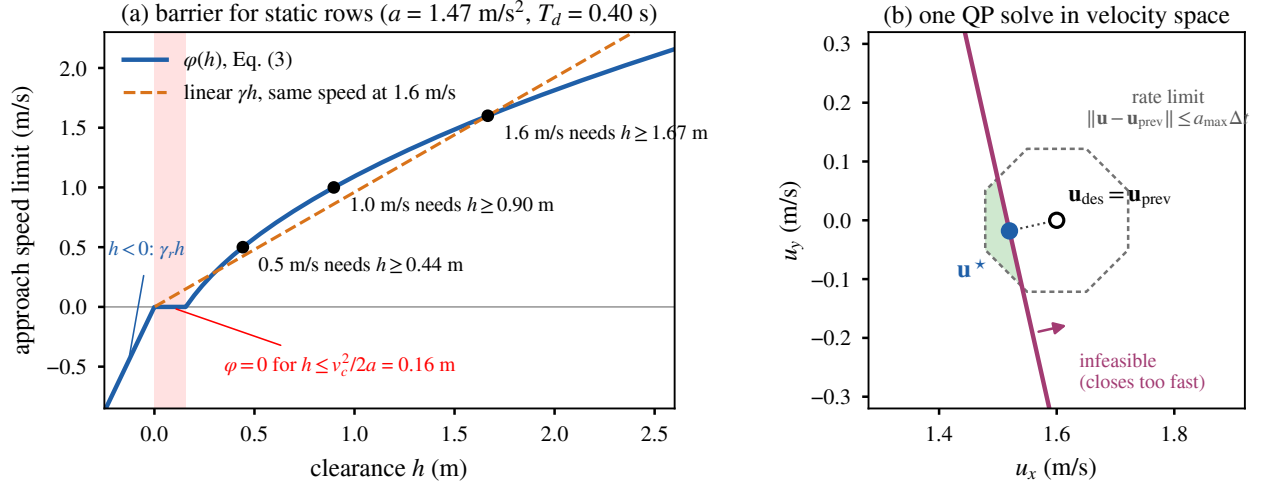
FIGURE 3. Mid-level safety filter with the mission parameters. (a) \varphi(h) of Eq. (3) for static rows: zero below h = 0.16 \text{ m} , and h \geq 1.67 \text{ m} is needed to approach at 1.6 m/s; a linear \gamma h equal at 1.6 m/s permits approach where \varphi demands a stop. (b) One QP solve by the flight code, illustrative case (east sweep at 1.6 m/s, mapped cylinder 2.51 m ahead, h = 1.49 \text{ m} ): the row of Eq. (4) cuts the rate-limited set, and the closing speed drops from 1.56 to 1.48 m/s.
